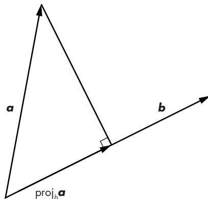
Figure 5-1: A graphical representation of the projection of a onto b in 2D
