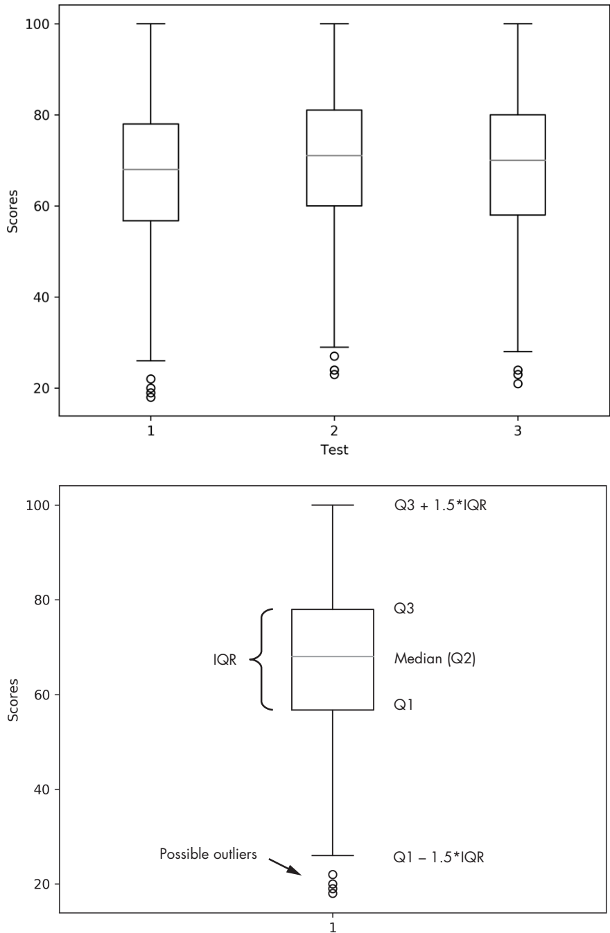
Figure 4-4: Box plots for the three exams (top), and the box plot for the first exam with the components marked (bottom)
