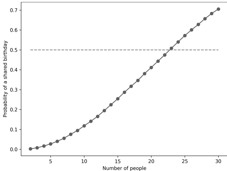
Figure 2-1: The probability of a shared birthday as a function of the number of people in a room
