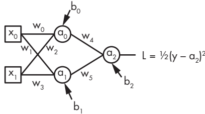
Figure 10-1: A simple neural network
